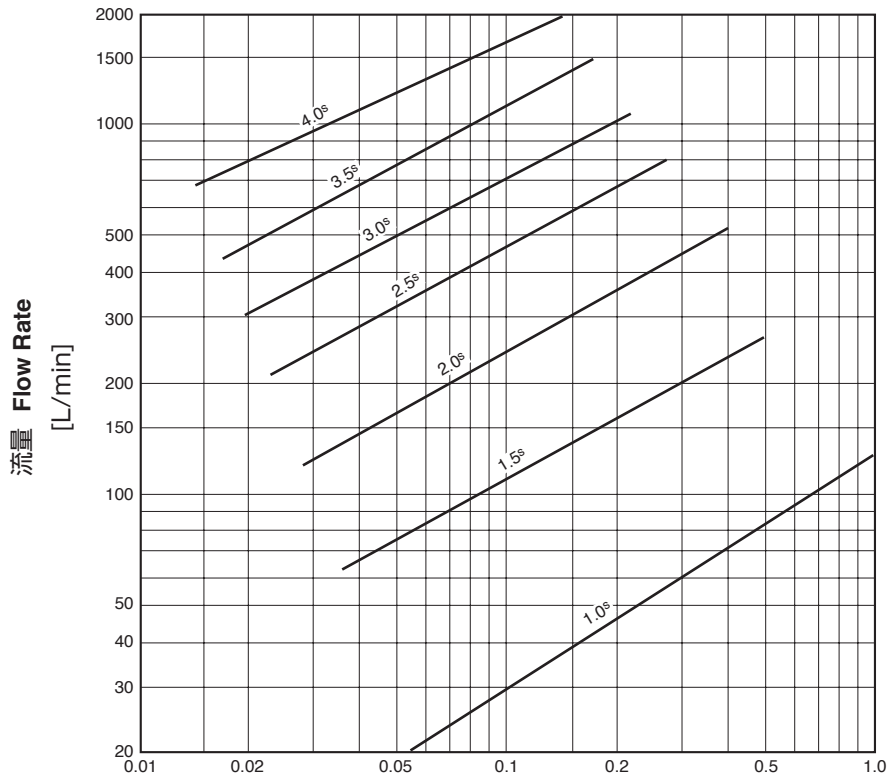
損失水頭 (パイプ1m当たり) Friction Head Loss — meter of Pipe Head(m)
